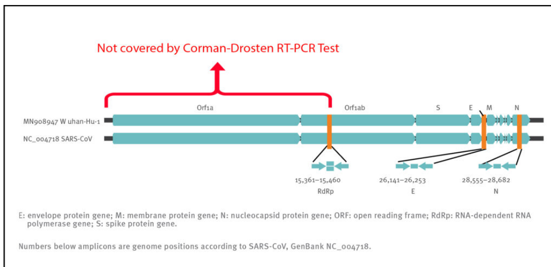
Figure 2: Relative positions of amplicon targets on the SARS coronavirus and the 2019 novel coronavirus genome. ORF: open reading frame; RdRp: RNA-dependent RNA polymerase. Numbers below amplicon are genome positions according to SARS-CoV, NC_004718 [1];
